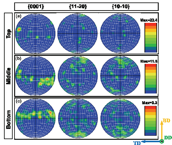
Fig. 5. Pole figures of different positions in SL component: (a) top; (b) middle; (c) bottom.
