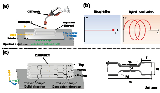
Fig. 1. Schematic of the experimental process for WA-DED AZ31 Mg alloy components: (a) deposition process; (b) deposition path; (c) position and size of the sample.
