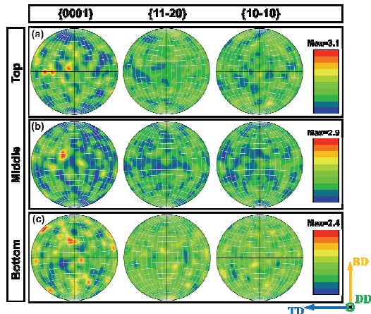
Fig. 6. Pole figures of different positions in SO component: (a) top; (b) middle; (c) bottom.
