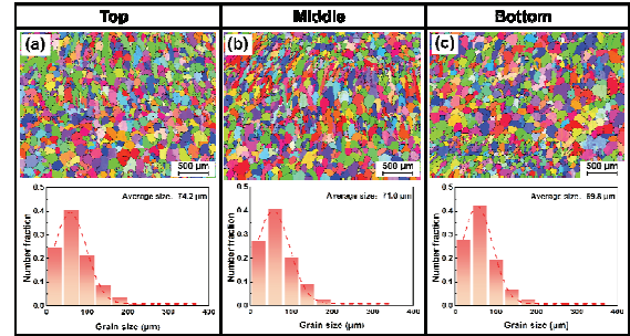
Fig. 4. IPF maps and grain size distribution histograms of different positions in SO component: (a) top; (b) middle; (c) bottom.
