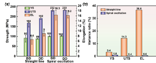
Fig. 2. Room temperature tensile property statistics: (a) performance statistics histogram; (b) histogram showing the rate of difference in performance comparison between BD and DD.
